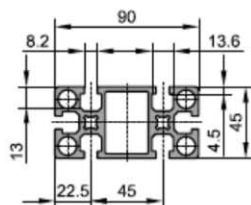
Profile cross-section
