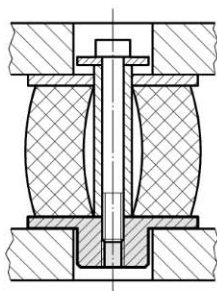
Mounting example
