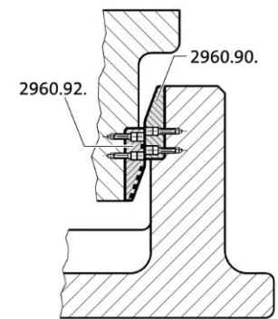
Mounting example
