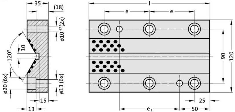
2963.72. Prismatic guide, Bronze with solid lubricant
